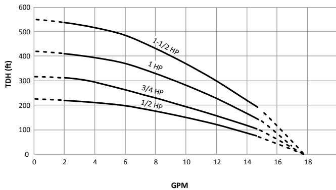
PUMP PERFORMANCE – 10 GPM
